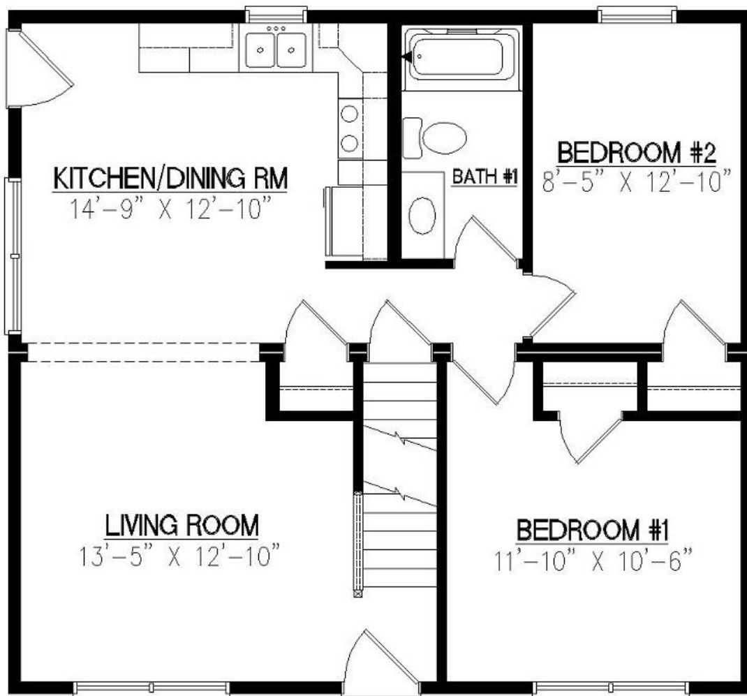
First Floor (w/ Basement)
